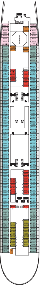
Deck 4 (Staterooms 4.001-4.225)
